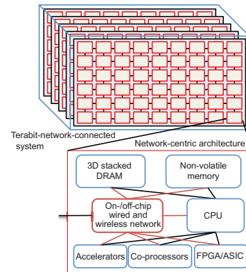
Fig. 1 Envisioned architectures for post-exascale systems
